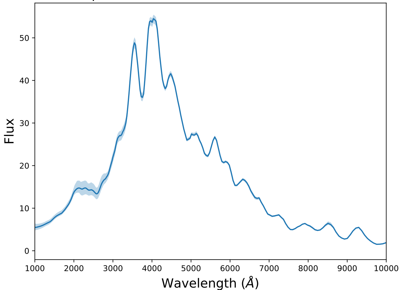
Spectrum 7 for transient SNIa at z=1.40
